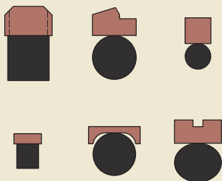
PTFE slide ring piston seals, profile examples
